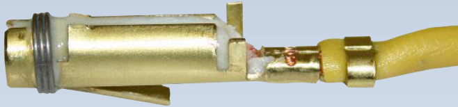
Heavy-duty brass with stainless compression ring
