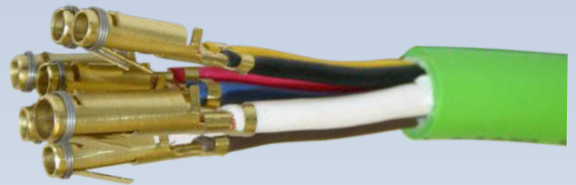
Conductor and insulation crimps
