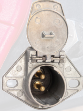
15-328 VERTICAL DUAL POLE INCLUDES 4 & 6 GA COPPER LUGS STD PKG: 5
