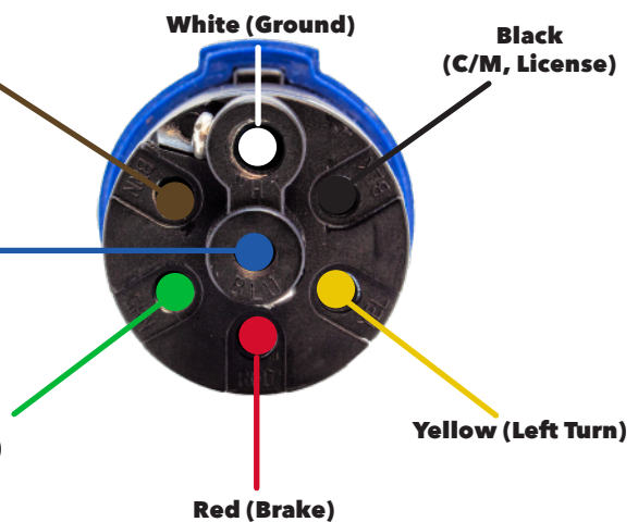
BACK OF PLUG INSERT
