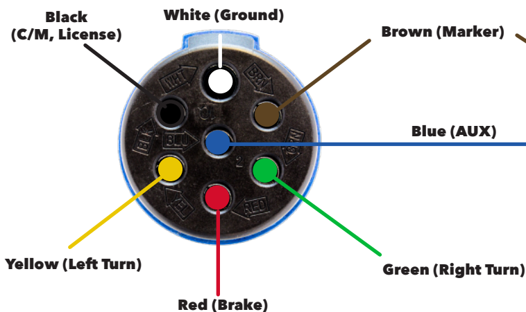
FRONT OF PLUG INSERT
