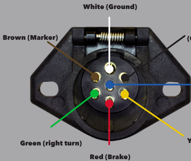
FRONT OF SOCKET
