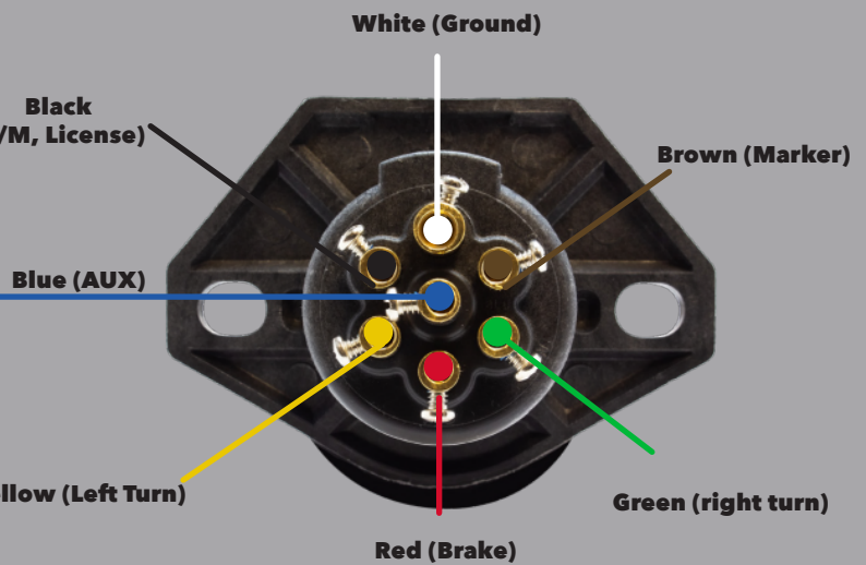
BACK OF SOCKET
